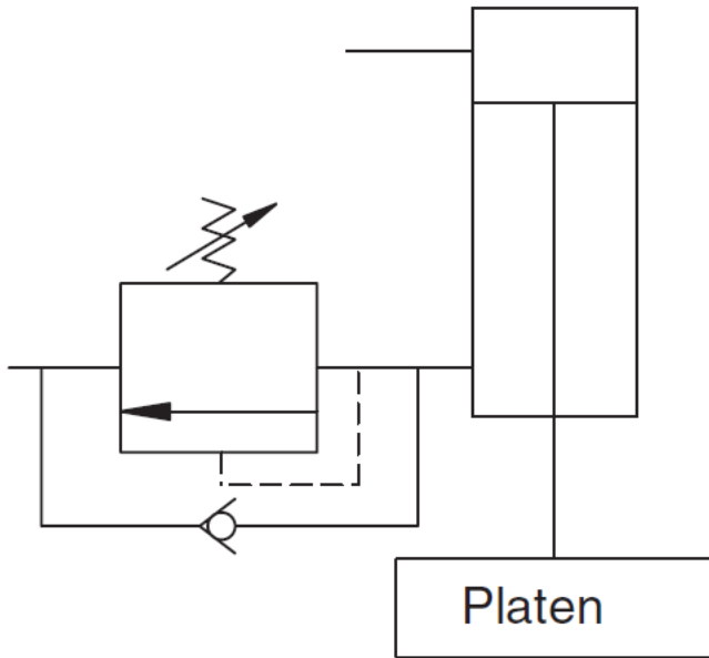
Valve Closed
