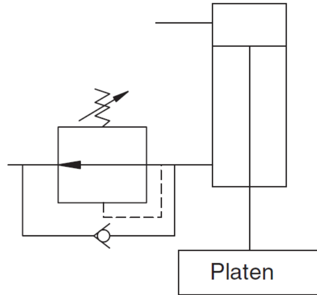
Valve Open
